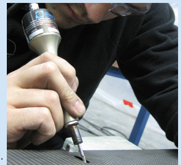
201SV 65,000 RPM, 0.2 HP 6 oz (0.17 kg)
